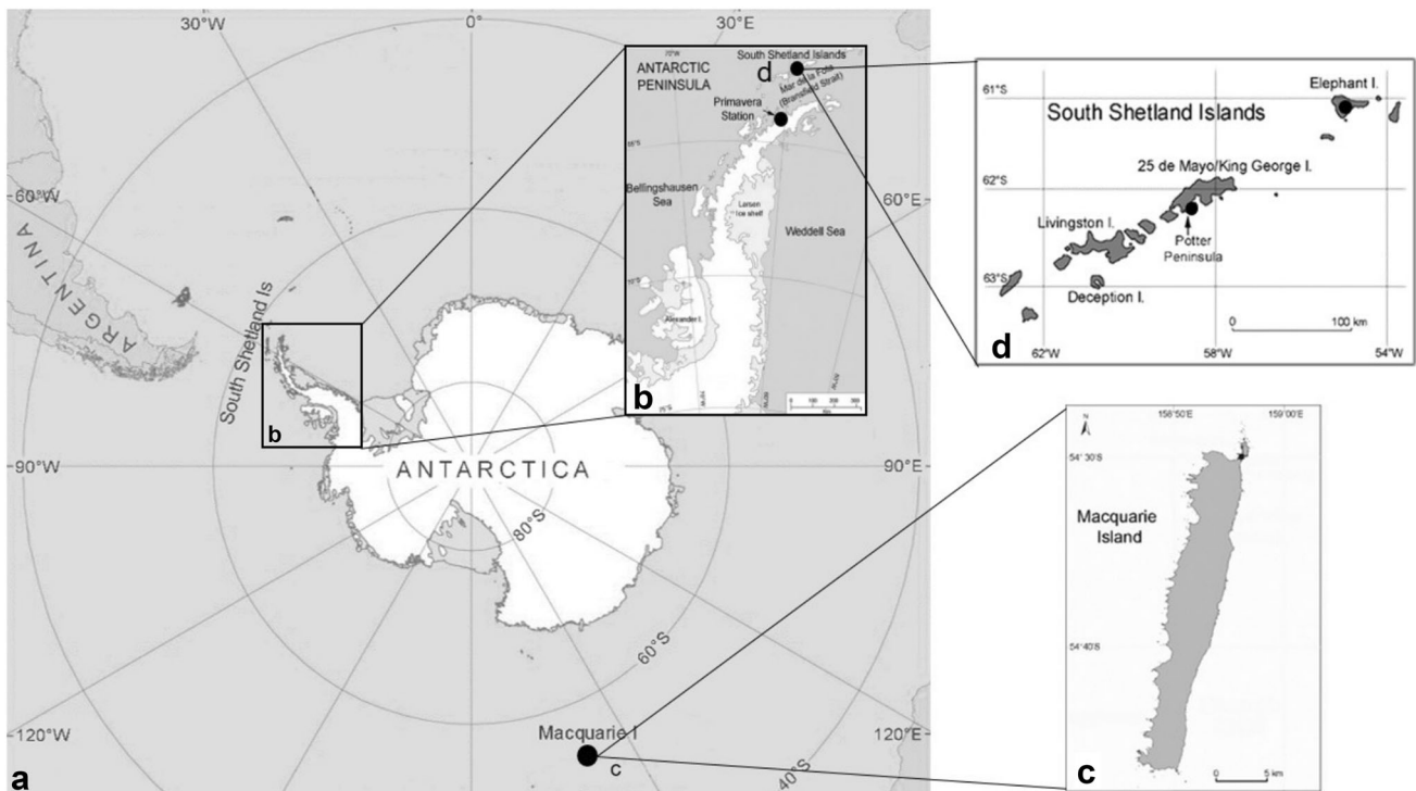
Fig. 2 Locations where Lepidophthirus macrorhini was reported. a General view of Antarctica; b Antarctic Peninsula, Base Primavera (present study), c Macquarie Island (Murray and Nicholls 1965),
