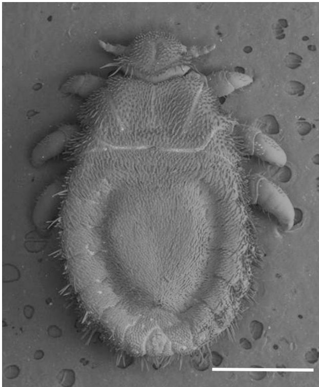
Fig. 1 Scanning electron microphotograph of the louse Lepidophthirus macrorhini from southern elephant seals (scale bar: 1 mm)
